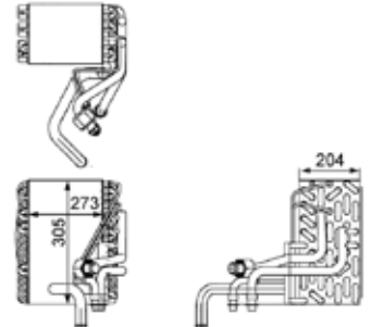
376753341 Radiator
