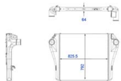
376761701 Charge Air Cooler
