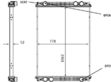
376761591 Radiator
