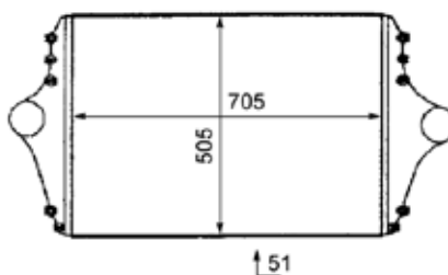
376730601 Charge Air Cooler
