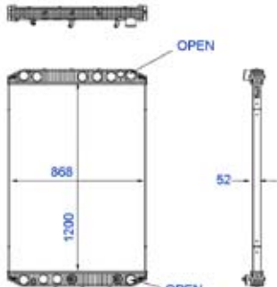
376761711 Charge Air Cooler
